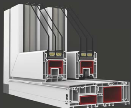
VEKA THRESHOLD standard 62 mm
