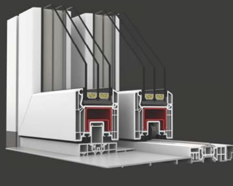
G-U THRESHOLD flatstep 24 mm
