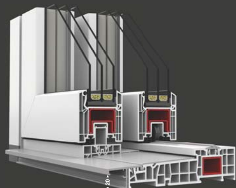
G-U THRESHOLD standard 50 mm
